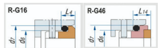
Single end seal R-HJ92N
