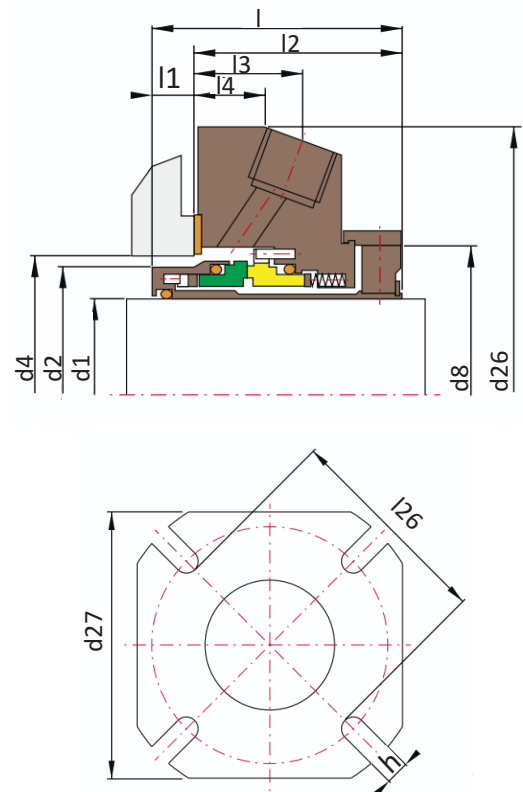
Mechanical seal R-TSSC-A05
