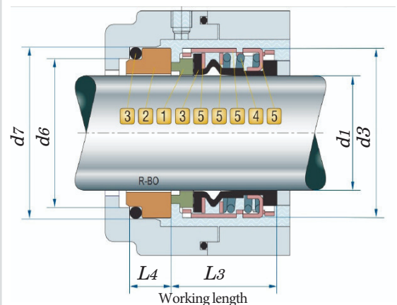
Single mechanical seal R-502
