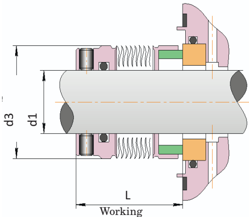
Mechanical end seal R-680 (676/ 670/ 680)
