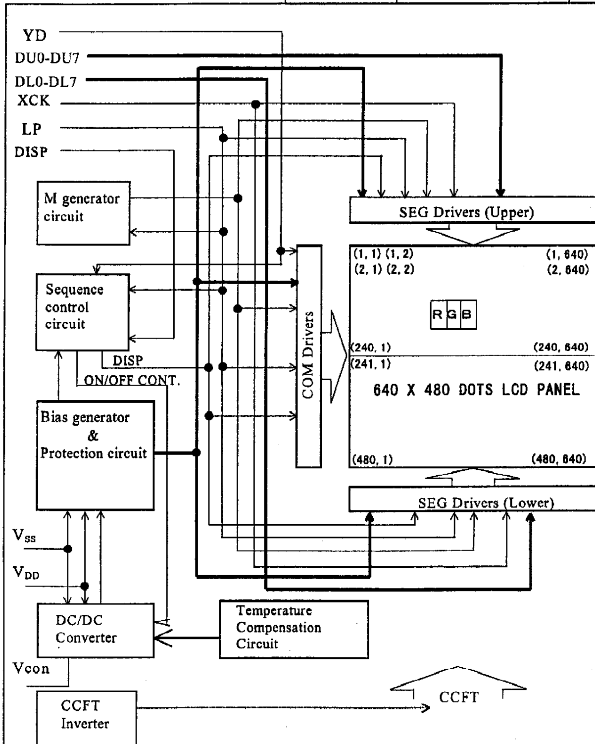
Fig. 10 Circuit block diagram
