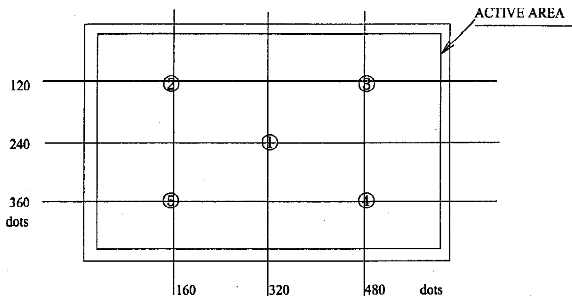
Fig.11 Measuring points (1-5)
