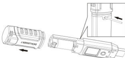
Figure 4 (Battery installment)
