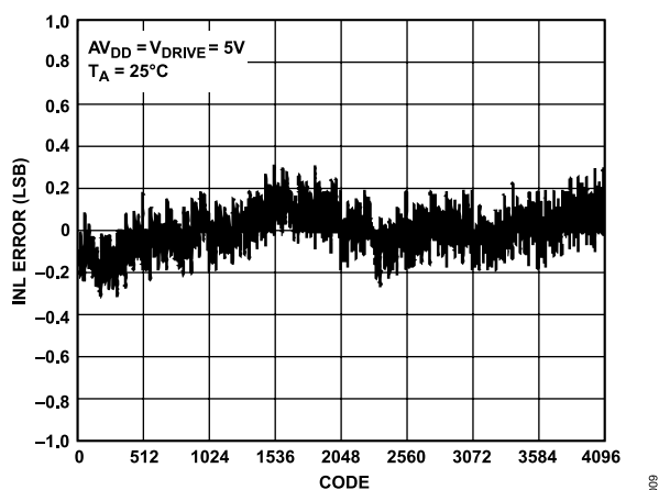
Figure 9. Typical INL
