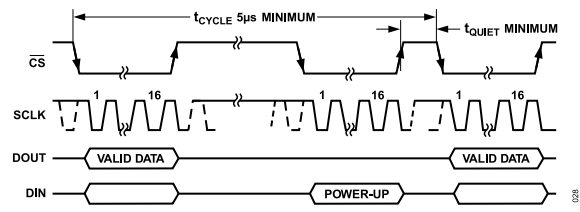
Figure 28. General Timing Diagram
