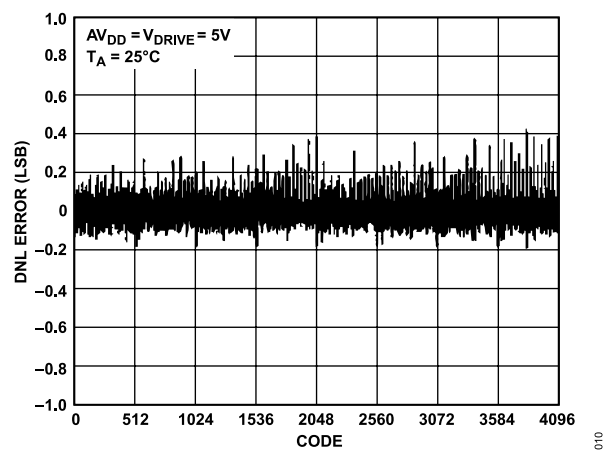
Figure 10. Typical DNL
