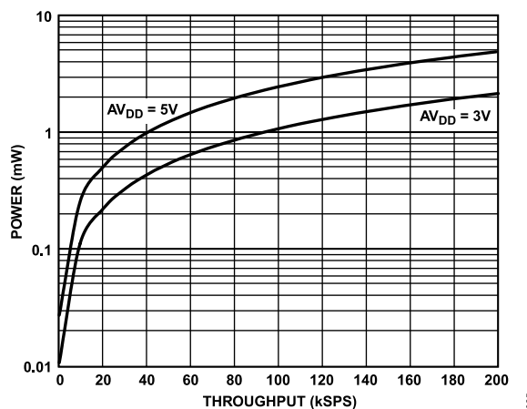
Figure 25. Power vs. Throughput Rate
