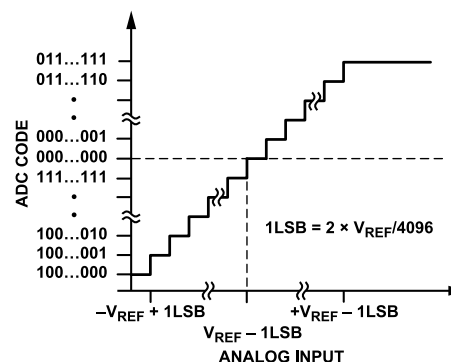
Figure 18. Twos Complement Transfer Characteristic with REF_{IN} \pm REF_{IN} Input Range
