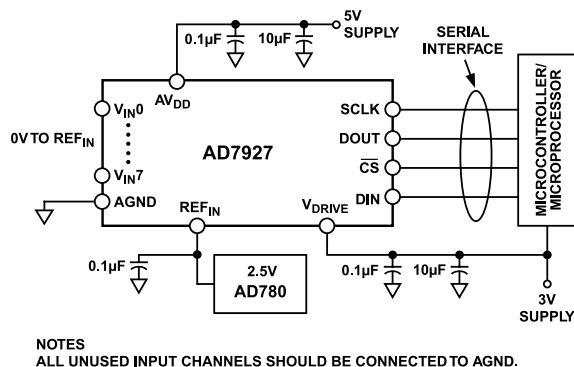
Figure 20. Typical Connection Diagram
