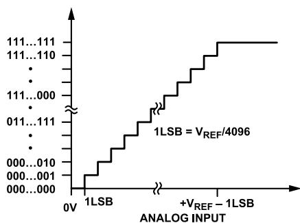
Figure 17. Straight Binary Transfer Characteristic
