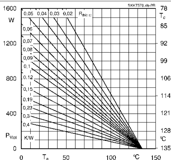
Fig. 2R: Max. power dissipation of one module vs. case temperature
