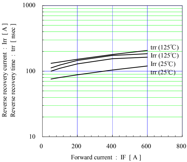
Reverse recovery characteristics (typ.) Vcc=300V, VGE=±15V, Rg=6.8Ω
