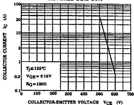
REVERSE BIAS SOA
