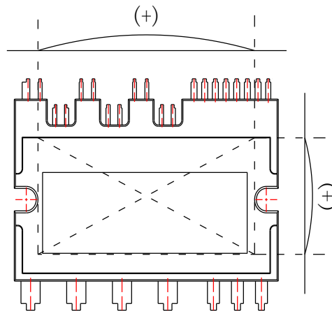
Fig 4. Flatness Measurement Position
