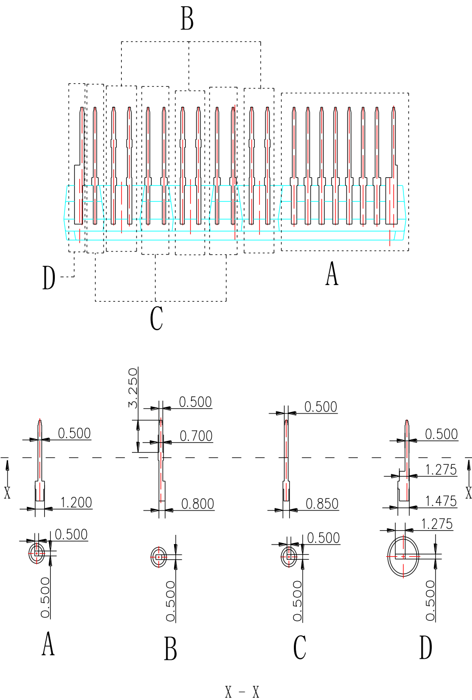
Fig 9.Detailed Package Outline Drawings
